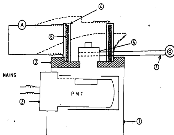
Fig 1.1 ML measuring device at different temperatures. PMT housing (2) Photomultiplier tube (3) Rubber sheet (4) Asbestos sheet and Al sheet (5) Lucite plate (6) Heating filament (7) Thermocouple (8) Variac
