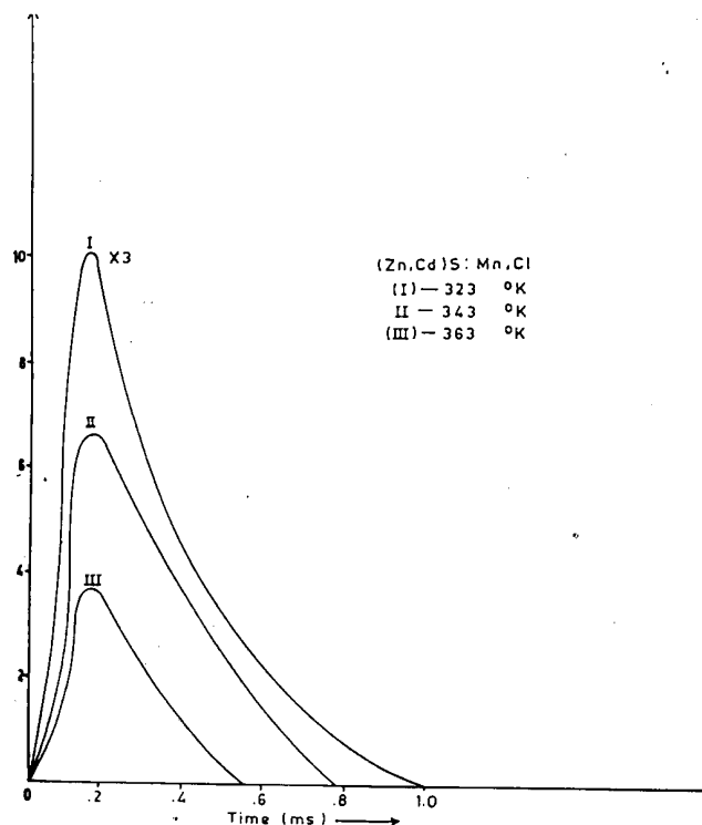
Fig 1.3 Time dependence of ML intensity of (Zn, Cd) S:Mn, Cl phosphors for different temperatures
