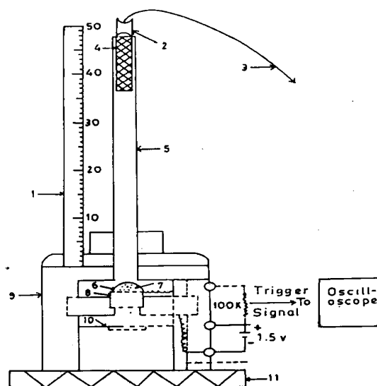
Fig 1.2 Schematic diagram of the experimental. Arrangement used for measuring the time dependence Of ML phosphors Scale in CMS, (2) Pulley, (3) Mettalic Wire (4) Load, (5) Guiding cylinder (6) Alluminium foil (7) Sample, (8) transparent Lucite plate, (9) Wooden block, (10) photomultiplier tube (11) Iron base mounted a table
