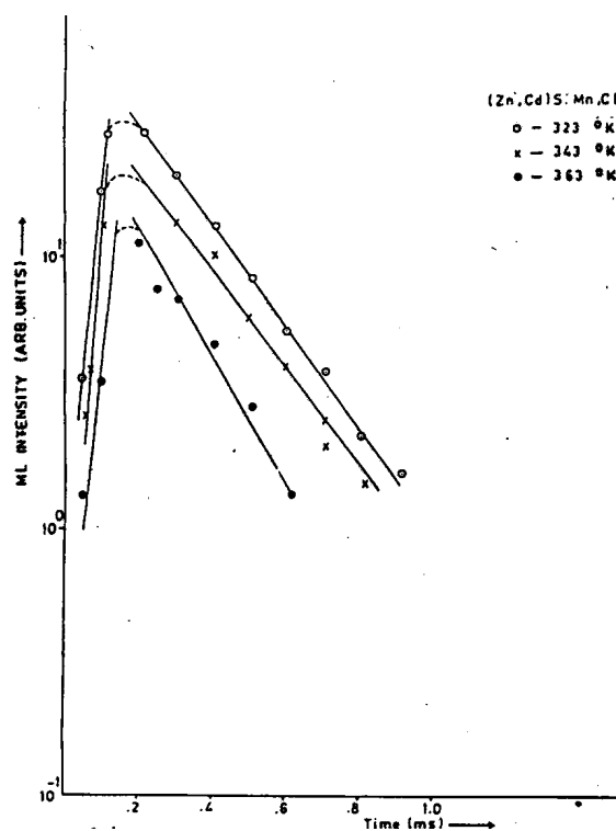
Fig 1.4 Plot of \log I versus t , for (Zn,Cd) S:Mn, Clphosphors at different temperatures
