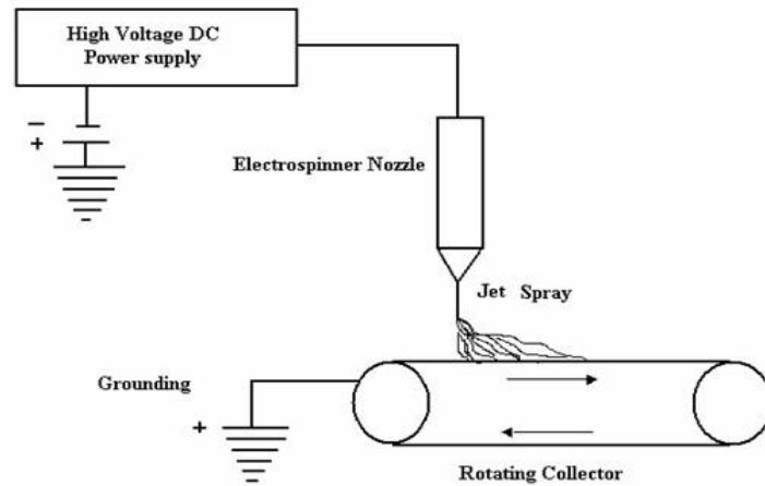
Schematic representation of electrospinning process
