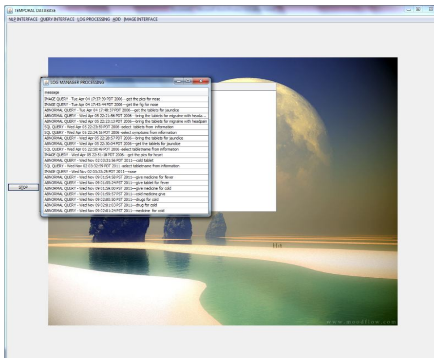
Figure 8: IQI Log details
