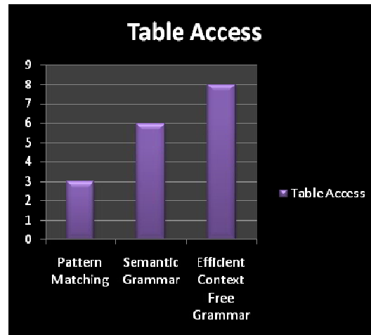
Figure 2: Performance Comparison for Table Access
